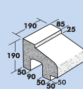
20.08 Sill (projecting)
