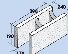
25.16 Open End Bond Beam Depressed Web
