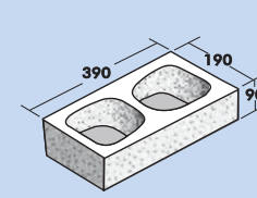
H20.04 Standard or Corner Half High
