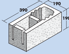
20.15 Corner Bond Beam
