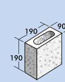
10.02 Half
