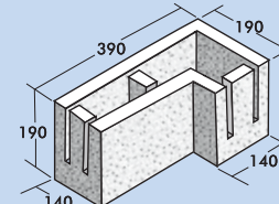
15.15 Right Hand Corner Bond Beam (Left hand also available)
