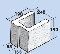
25.11 Rebate Lintel
