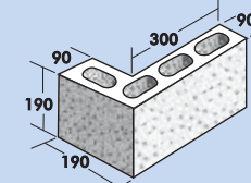
10.03 Corner
