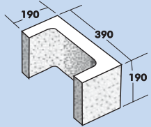
20.34 Pilaster 'C' Type
