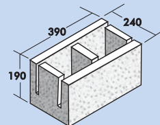
25.14 Knock-in Bond Beam
