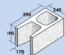
25.05 Open End and Plain End
