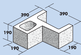
20.35 Pilaster 'H' Type
