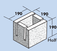
20.44 Knock-in Half Bond Beam
