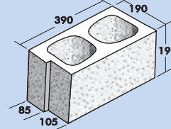
20.09 Rebate Whole
