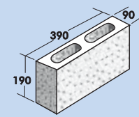
10.01 Standard Whole
