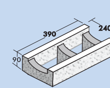
H25.14 Bond Beam Depressed Web
