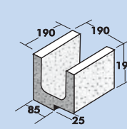
20.11 Rebated Lintel
