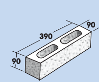
H10.01 Standard Whole
