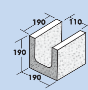
20.12 Lintel and Half-end Closer
