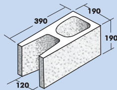
20.05 Open End
