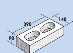
H15.04 Half High Standard
