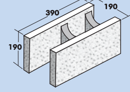
20.16 Open End Bond Beam Depressed Web
