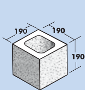
20.02 Half
