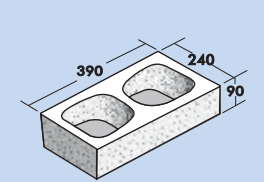
H25.04 Standard or Corner Half High
