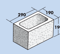
20.19 Three Quarter
