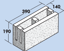
15.14 Knock-in Bond Beam
